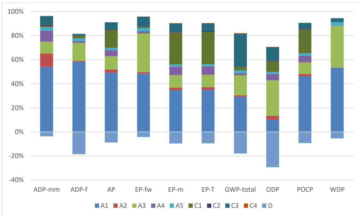
Figure 2: Tensor® RE560 - Impact of the individual modules on the environmental core indicators
